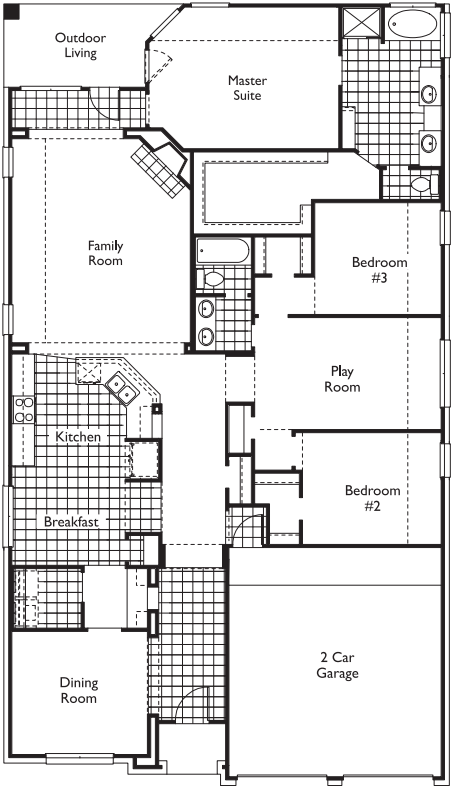
Lower Level
